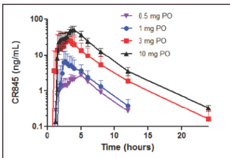
Figure 11: Phase 1a Pharmacokinetic Profiles of Ascending Concentrations of CR845 Capsules in Human Subjects.
